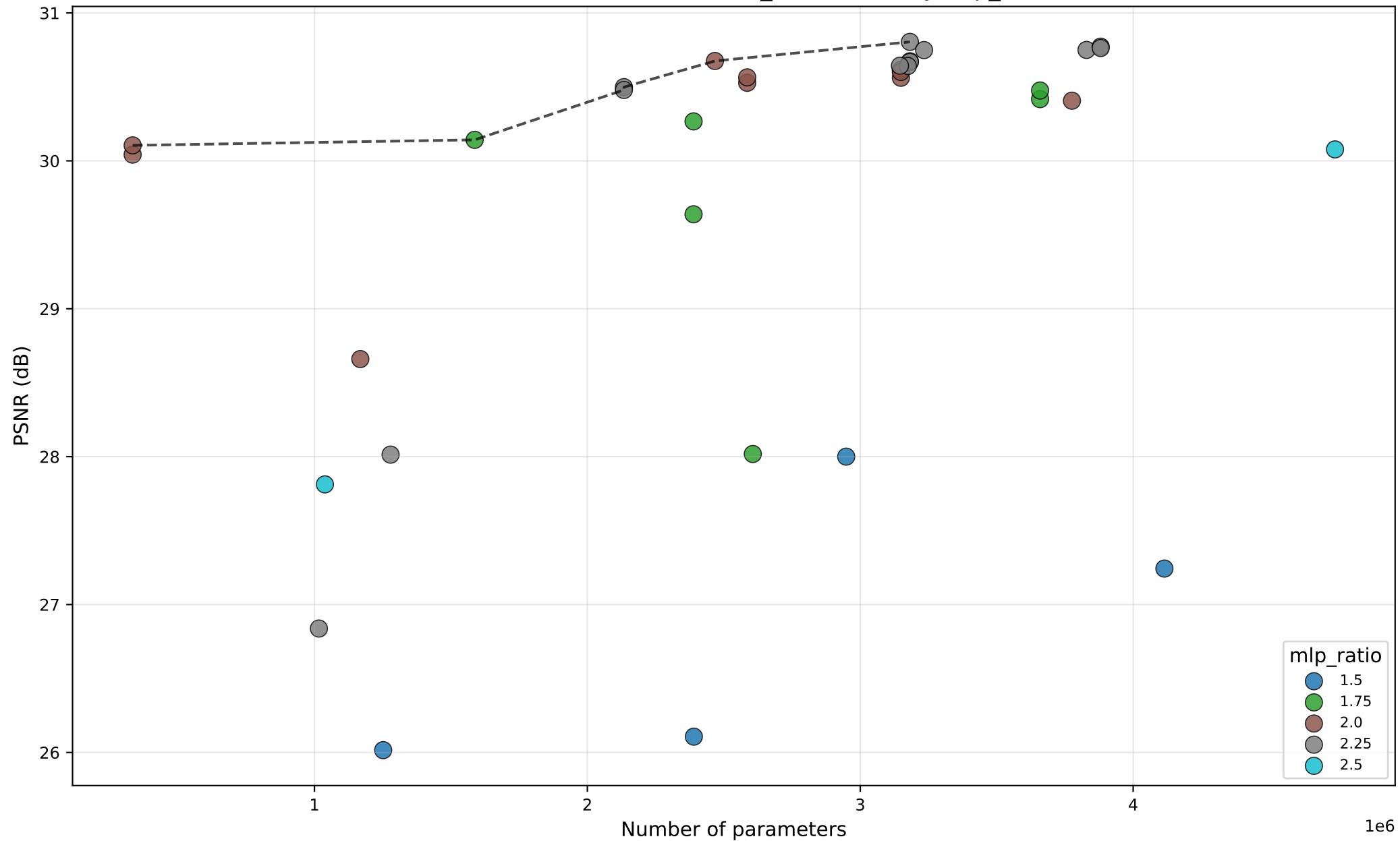
PSNR vs #Params — DHTCUN_baseline — by mlp_ratio
